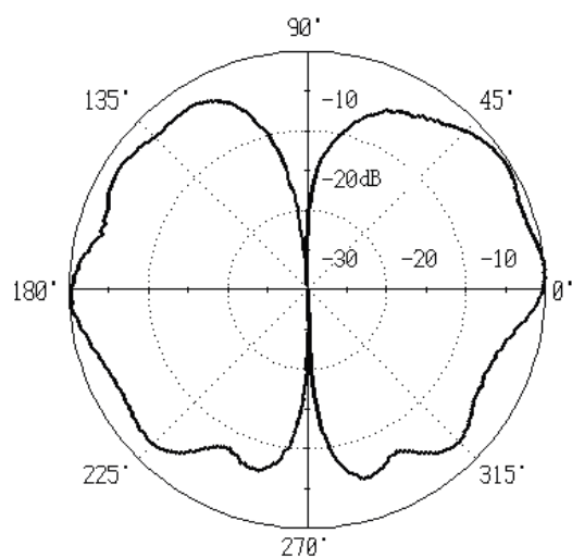
E Plane
